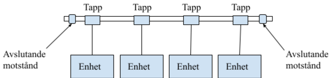
Figur 2.10: ControlNet trunkline-dropline
